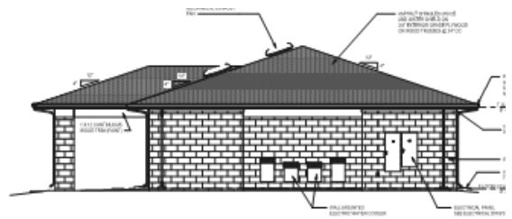
EAST ELEVATION
