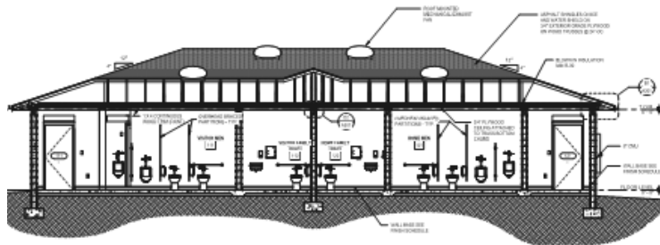
BUILDING CROSS SECTION - VISITOR MEN/MEN
