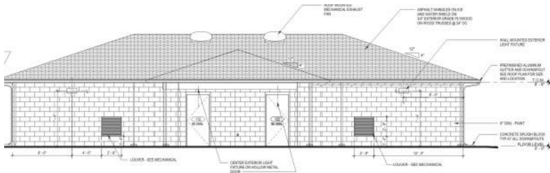
7 SOUTH ELEVATION 1/4" = 1'-0"
