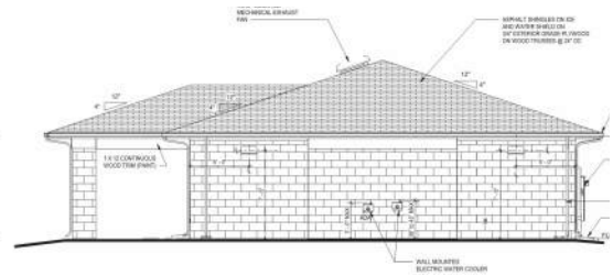
8 EAST ELEVATION 1/4" = 1'-0"
