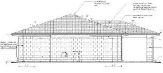
10 WEST ELEVATION 1/4" = 1'-0"
