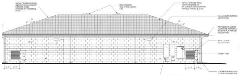
9 NORTH ELEVATION 1/4" = 1'-0"
