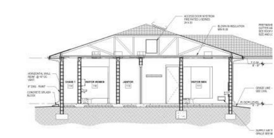
12 BUILDING CROSS SECTION 1/4" = 1'-0"
