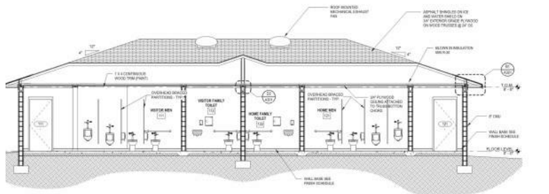
11 BUILDING CROSS SECTION - VISITOR MEN/HOME MEN 1/4" = 1'-0"
