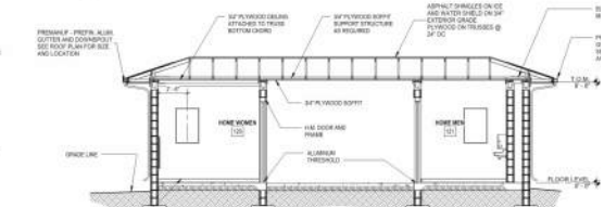
14 BUILDING CROSS SECTION 1/4" = 1'-0"
