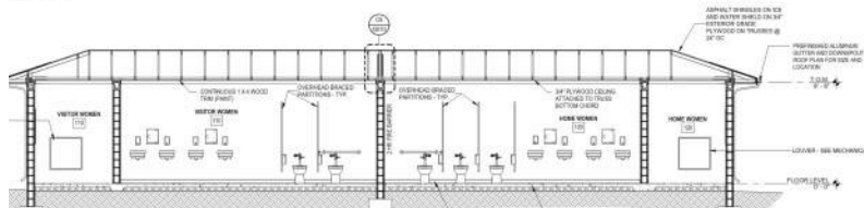
13 BUILDING CROSS SECTION - VISITOR WOMEN/HOME WOMEN 1/4" = 1'-0"
