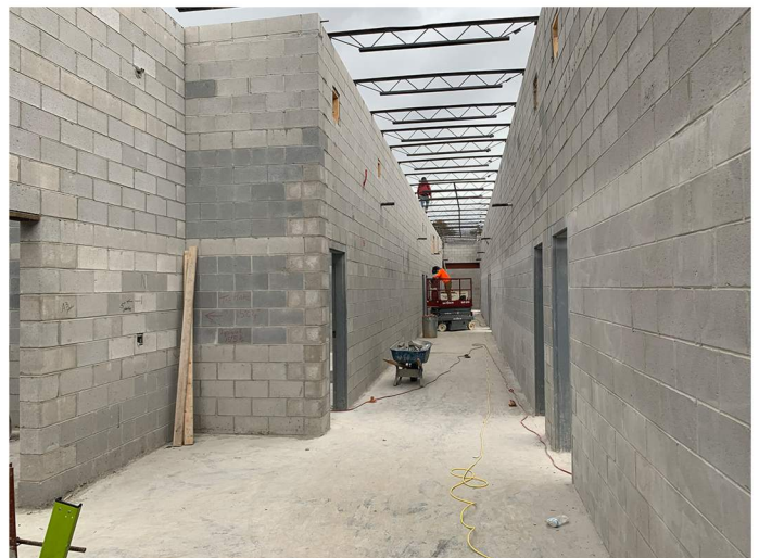
Steel joint installation is in progress.
