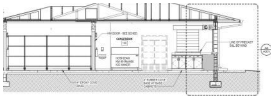
BUILDING SECTION 1/8" = 1'-0"
