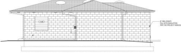
EAST ELEVATION 1/8" = 1'-0"
