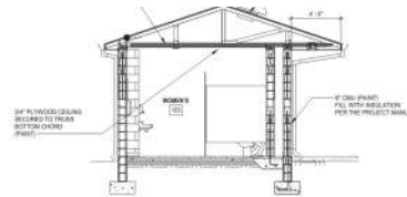
BUILDING SECTION 1/8" = 1'-0"
