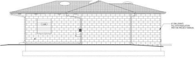
EAST ELEVATION 1/8" = 1'-0"
