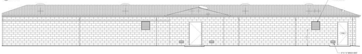
WEST ELEVATION 1/8" = 1'-0"
