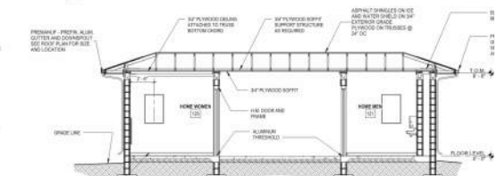
12 BUILDING CROSS SECTION 1/4" = 1'-0"
