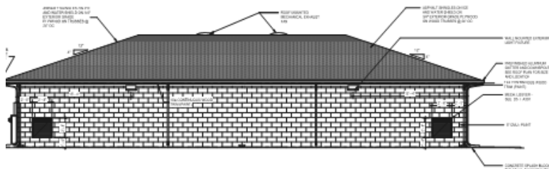
NORTH ELEVATION SECTION
