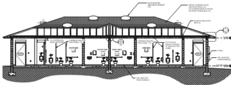
BUILDING CROSS SECTION - VISITOR MEN/MEN SECTION
