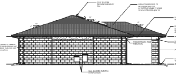
WEST ELEVATION SECTION
