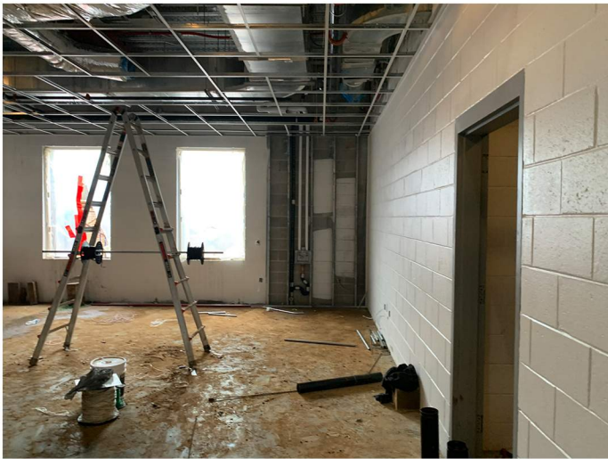
Ceiling grid installation is in progress.
